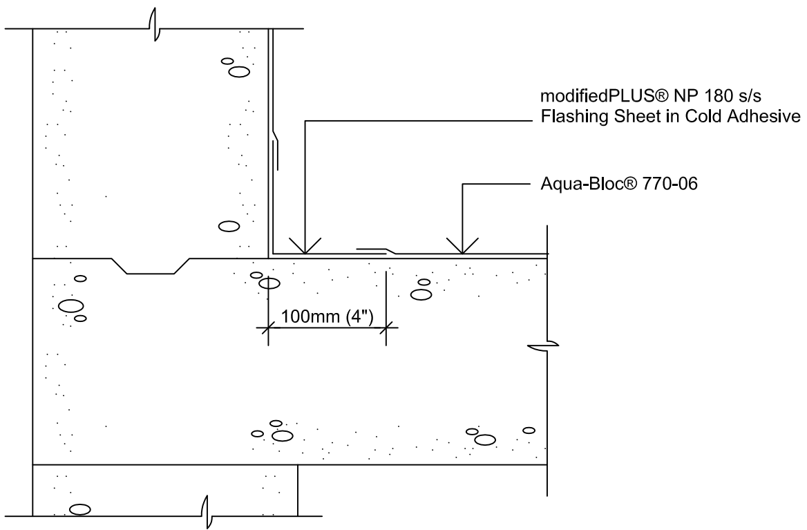
Non-Monolithic Deck to Wall Juncture
