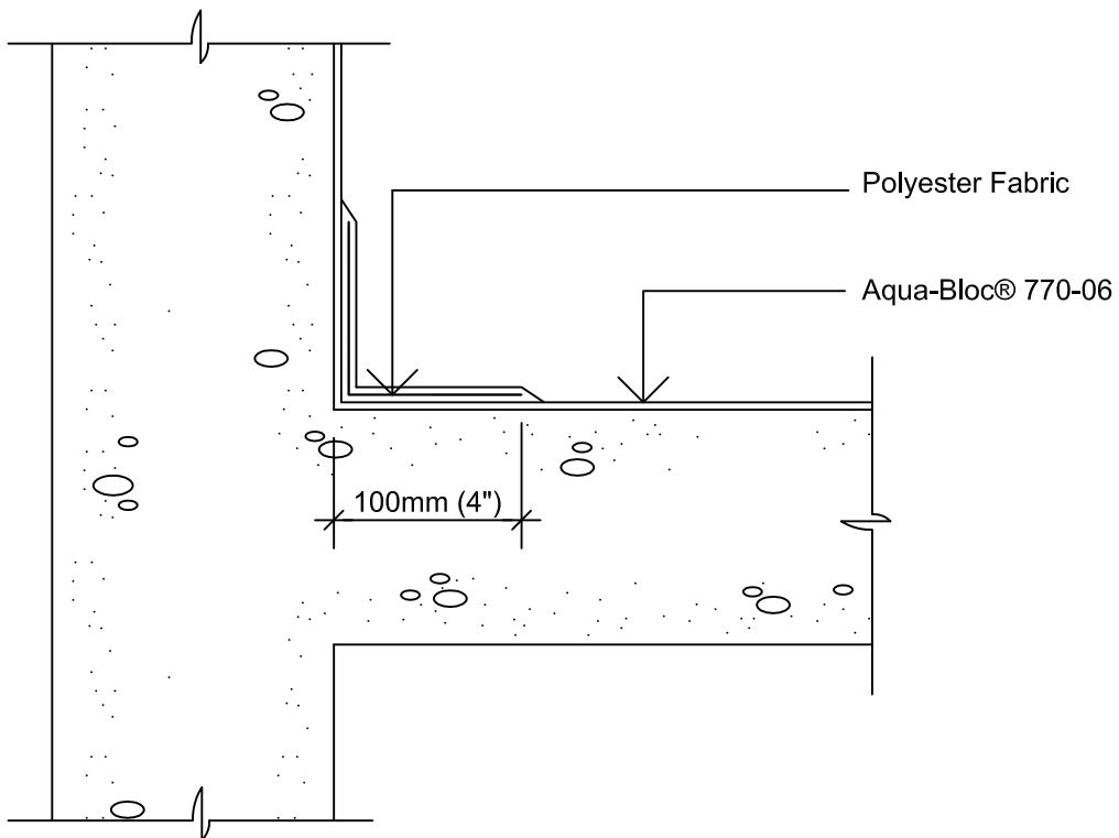
Monolithic Deck to Wall Juncture
