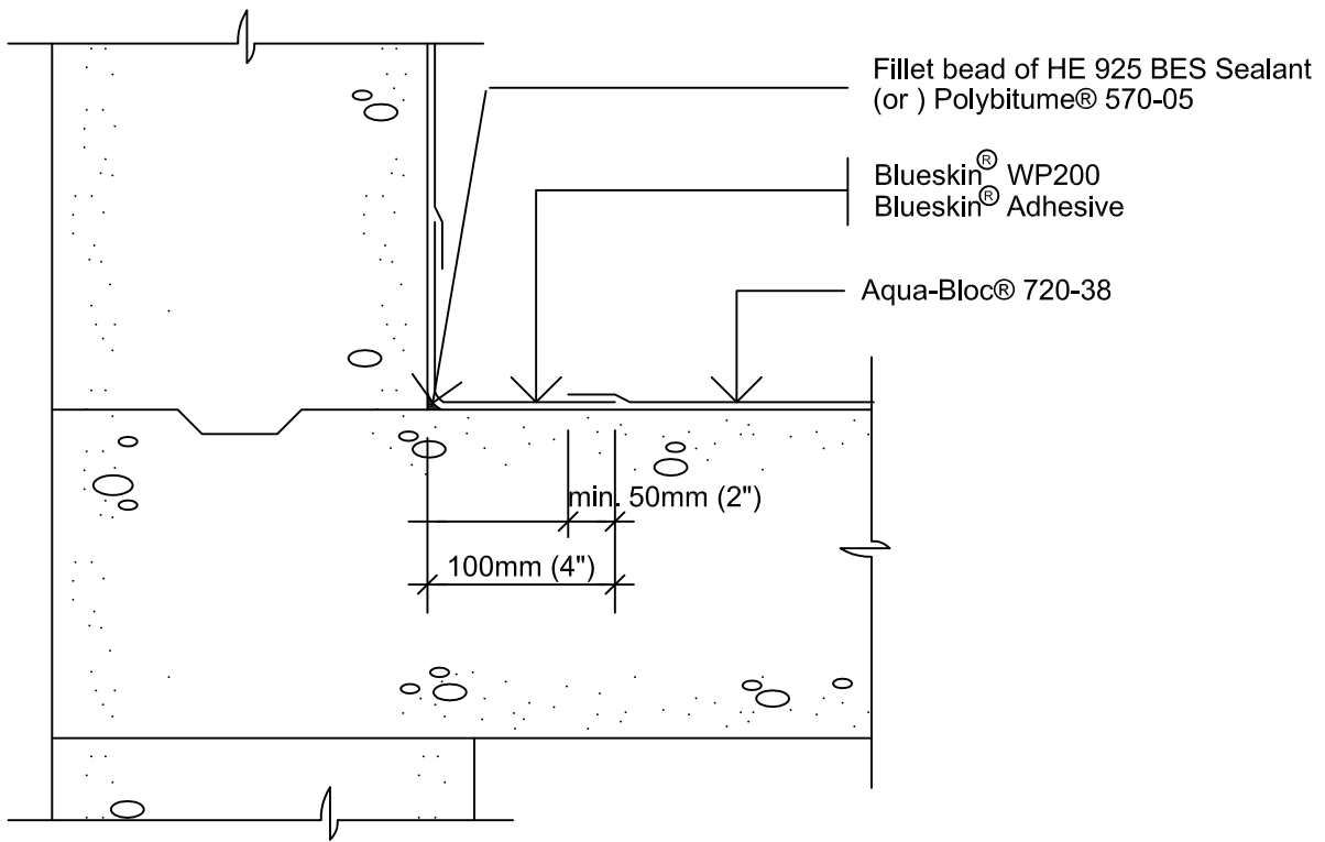
Non-Monolithic Deck to Wall Juncture
