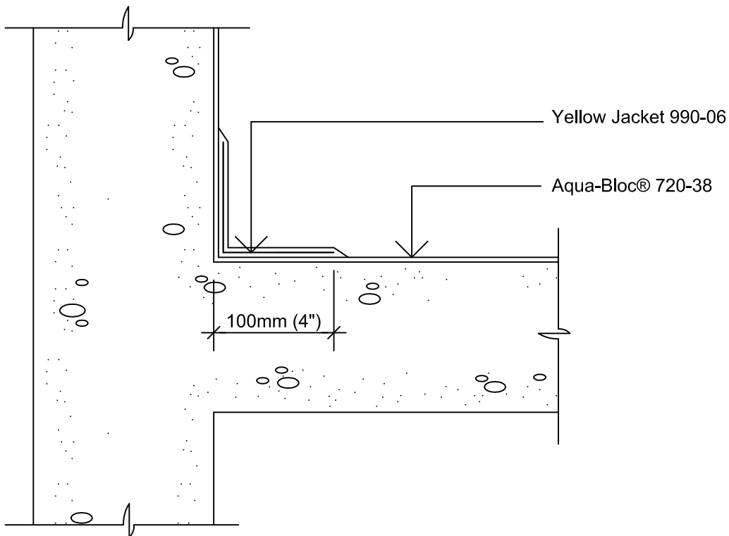
Monolithic Deck to Wall Juncture
