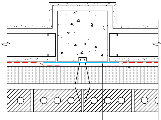
Blueskin SA Transition Sheet Air-Bloc 17MR Concrete Column
