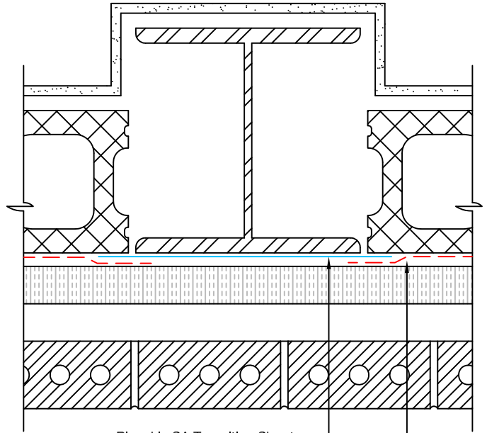
Blueskin SA Transition Sheet Air-Bloc 17MR Steel Column
