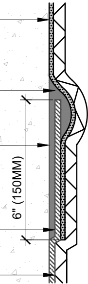
METHOD #2 - TERMINATION SEALANT TEMPORARILY SECURED MEMBRANE
