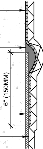
METHOD #1 - TERMINATION SEALANT FULLY BONDED MEMBRANE
