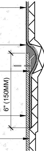
METHOD #3 - TERMINATION SEALANT TEMPORARILY SECURED MEMBRANE
