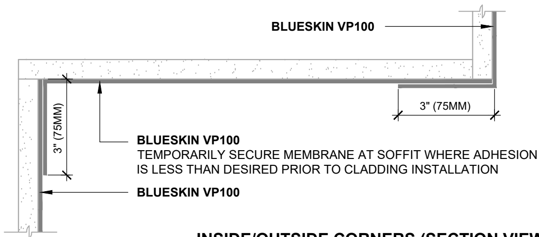
INSIDE/OUTSIDE CORNERS (SECTION VIEW) WRB WRAPPED AROUND CORNER
