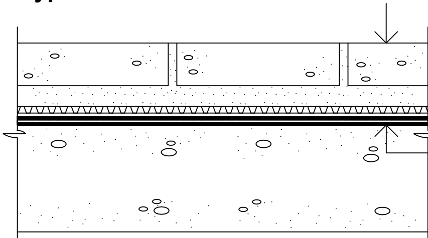
Typical Plaza (Pavers in Setting Bed)
